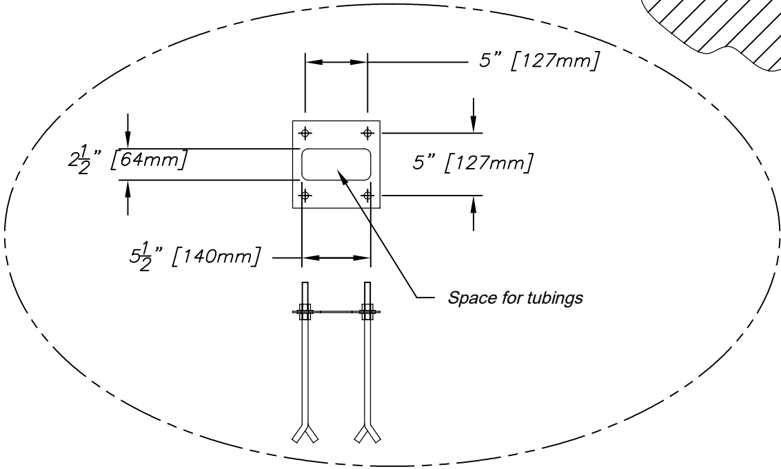
Installation template details
