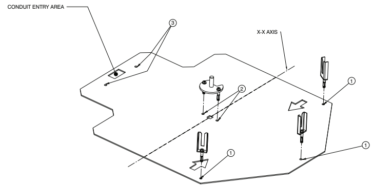
DRILLING TEMPLATE POSITIONING (ITEM 0/1924/128) 3D VIEW
