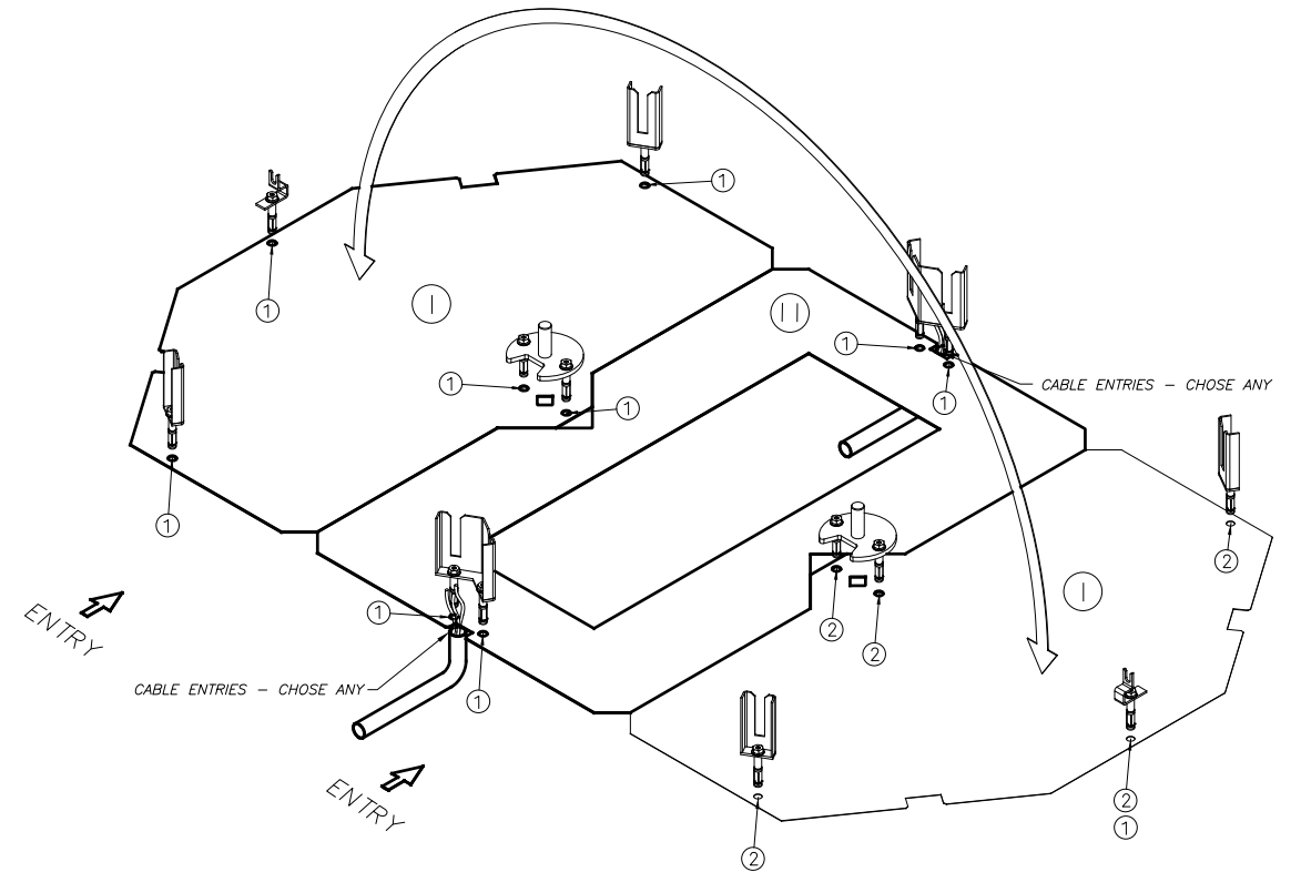
POSITIONING TEMPLATE ITEM NO. GBR-E-0007770 & GBR-E-0007773
